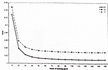
Fig. 9. Ability to learning new data using: (1) Hybrid algorithm topology; (2) Best random topology; (3) Hybrid algorithm topology but 100% connected.
